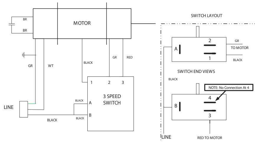
E85507 Carpet Drier Switch Layout & Wiring Diagram
